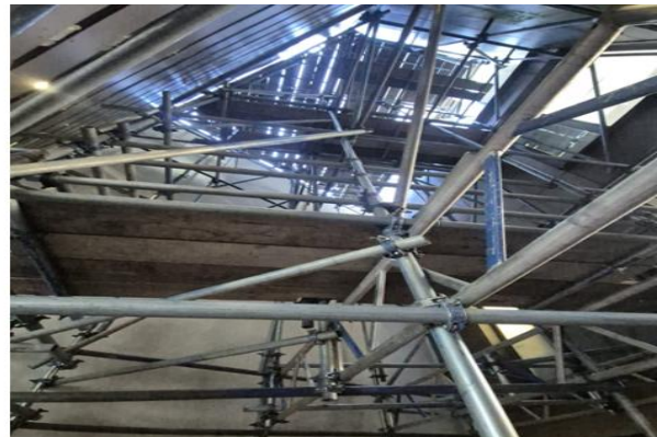
A photo showing Crash Deck Scaffold At 90% and in progress to completion
